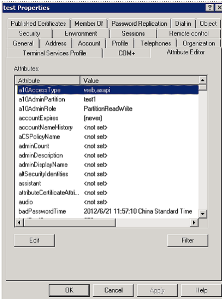
Figure 15 : Changing the Access Type
