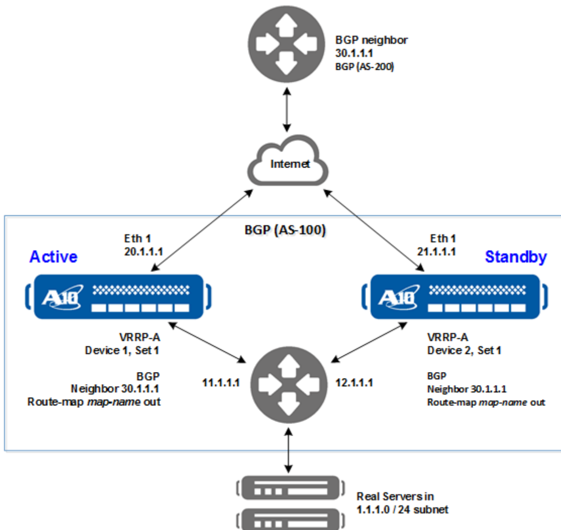
Figure 12 : Topology Using BGP Route Map (with VRRP-A High Availability Matching)
