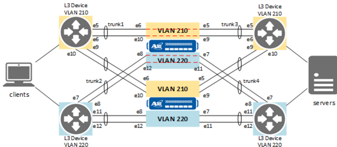
Figure 1 : LACP Passthrough - Example Topology
