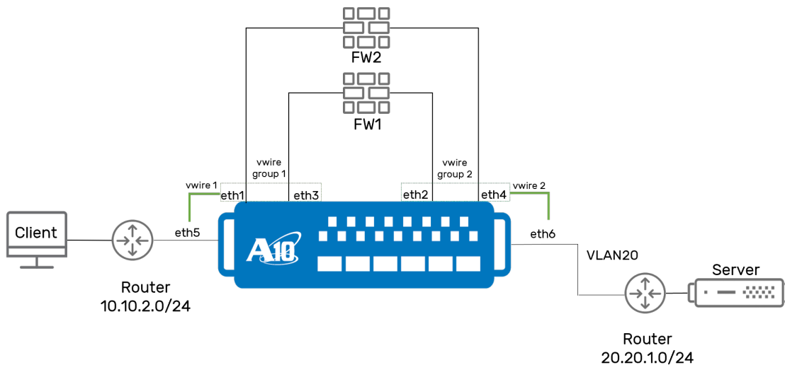
Figure 8 : Virtual Wire Firewall Deployment Example
