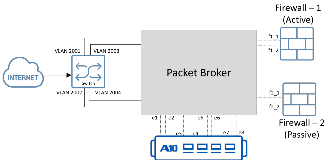
Figure 9 : Virtual Wire SSLi Firewall Deployment Example
