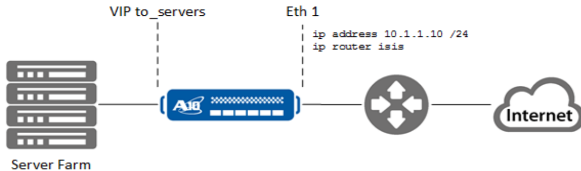
Figure 11 : ACOS Device in a Basic IS-IS Topology
