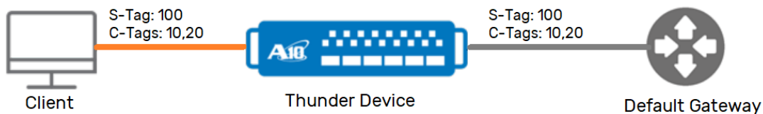
Figure 3 : Double tagged transit traffic
